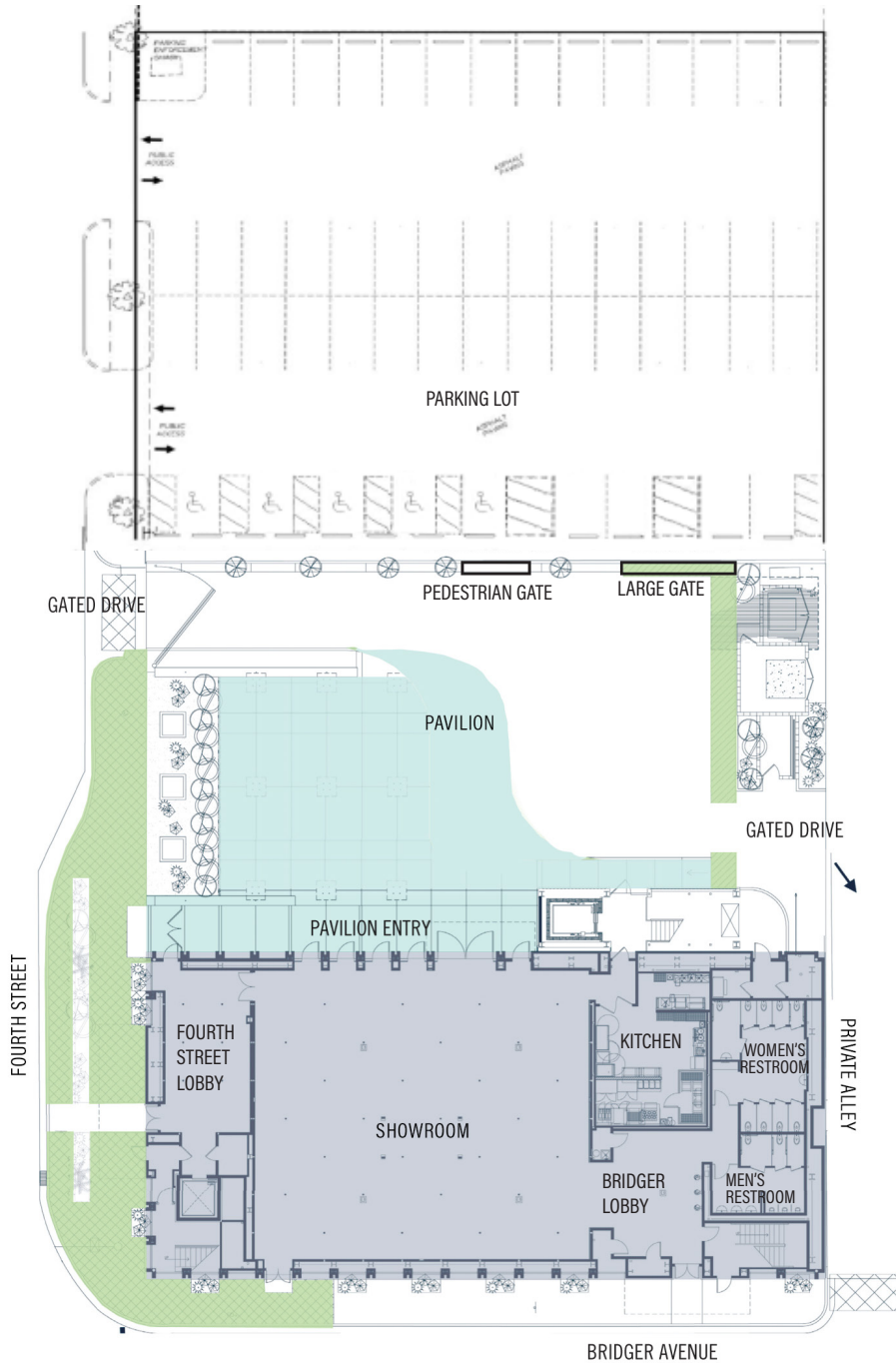
SHOWROOM/PAVILION/PARKING
